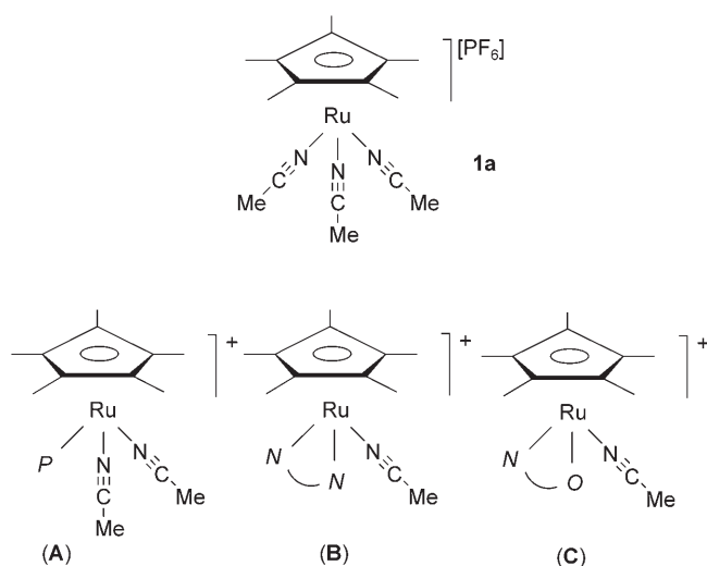
Scheme 1. Ruthenium(II) precatalysts related to complex 1a : (A) P=P(\text{OMe})\text{Ph}_2 , P(o\text{-tolyl})\text{Ph}_2 ; (B) N,N=2,2' -bipyridine or \alpha -diimine type ligands; (C) N,O=2 -quinolinecarboxylic acid.
