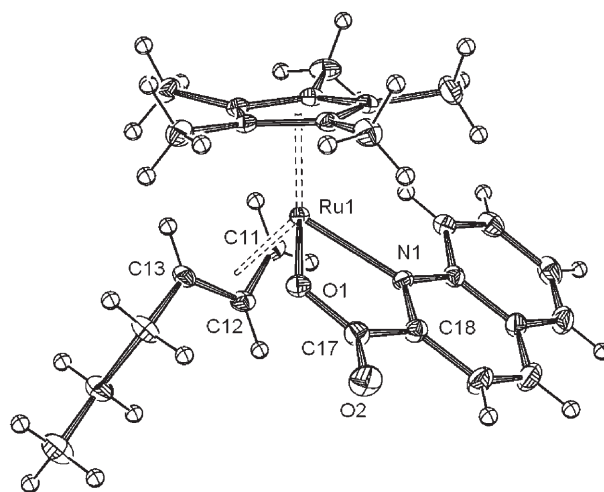
Figure 2. ORTEP drawing of 4a showing 50% probability thermal ellipsoids. The \text{BF}_4 anion and the \text{CH}_2\text{Cl}_2 molecule are omitted for clarity. Selected bond lengths [Å] and angles [°]: Ru1–O1 2.065(1), Ru1–N1 2.165(2), Ru1–C11 2.195(2), Ru1–C12 2.168(2), Ru1–C13 2.315(2), C11–C12 1.408(3), C12–C13 1.400(3); O1–Ru1–N1 77.40(6), O1–Ru1–C13 80.34(7), N1–Ru1–C11 87.07(7), O1–Ru1–C11 127.17(7), N1–Ru1–C13 118.98(7), C11–Ru1–C13 63.88(8).
