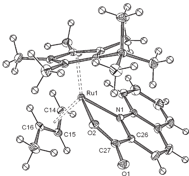
Figure 1. ORTEP drawing of 3b showing 50% probability thermal ellipsoids. The \text{PF}_6 anion is omitted for clarity. Selected bond lengths [Å] and angles [°]: Ru1–O2 2.056(1), Ru1–N1 2.173(2), Ru1–C14 2.196(2), Ru1–C15 2.176(2), Ru1–C16 2.327(2), C14–C15 1.418(3), C15–C16 1.404(3); O2–Ru1–N1 76.87(5), O2–Ru1–C16 78.45(6), N1–Ru1–C14 85.96(6), O2–Ru1–C14 126.04(6), N1–Ru1–C16 116.39(6), C14–Ru1–C16 64.33(7).
