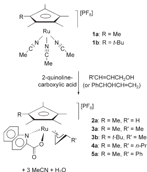
Scheme 2. Synthesis of [\text{Ru}(\text{C}_5\text{Me}_4\text{R})(2\text{-quinolinecarboxylato})(\eta^3\text{-allyl})][\text{PF}_6] complexes.
